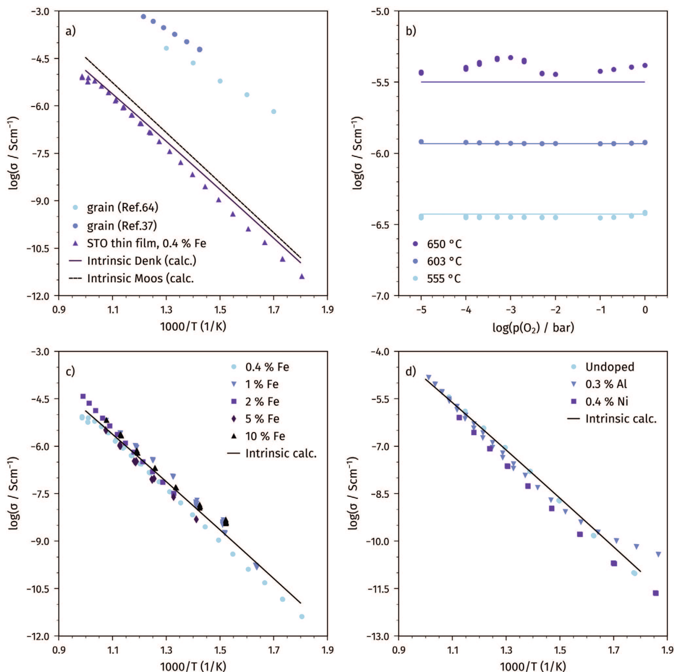
Figure 2. DC conductivity obtained from the DC resistance of doped SrTiO 3 thin films, measured by electrochemical impedance spectroscopy. a) Comparison of DC conductivities of thin films deposited from a 0.4% Fe doped target to the expected conductivity of bulk samples [37,64] and to the calculated conductivity of pseudo-intrinsic electronic conductivity ( [h^+] = [e'] ). [1,2] b) oxygen partial pressure dependence of the conductivity of a Fe-doped thin film deposited from a target with 0.4% Fe at three different temperatures (555 °C, 603 °C and 650 °C). No variation of the conductivity is observed in an oxygen partial pressure range from 10 -5 to 1 bar oxygen, the conductivity is close to the pseudo-intrinsic conductivity calculated from literature. [1] c) DC conductivity of Fe-doped SrTiO 3 thin films deposited from targets with different doping concentrations ranging from 0.4% up to 10% together with the electronically intrinsic conductivity ( [h^+] = [e'] ). [1] d) DC conductivity of nominally undoped SrTiO 3 thin films and slightly acceptor doped thin films with different doping ions (Ni or Al).
