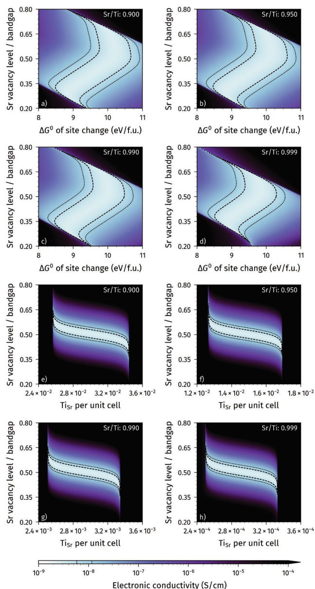
Figure 11. a) to d) Contour plots of the electronic conductivity at 400 °C, p_{O_2} = 1 bar for undoped SrTiO 3 thin films of different Sr/Ti ratios for different V_{Sr} levels in the band gap and different standard Gibbs free energies of the site change reaction \Delta G^0 . The inner bold dashed lines indicate the region in which the conductivity is less than a factor of two above the intrinsic conductivity (i.e. for [e'] = [h'] ), the outer dashed lines indicate a factor of four. The calculations are done in two steps: First, the equilibrium Ti_{Sr} concentration is calculated under PLD conditions (650 °C, 0.15 mbar O_2 ). Then, the Ti_{Sr} concentration is taken as frozen-in and all other defect concentrations are recalculated for 400 °C. Sr vacancies around mid-gap and \Delta G^0 around 10 eV cause pseudo-intrinsic behavior for a very broad range of Sr/Ti ratios. e) to h) Contour plots indicating the electronic conductivity at 400 °C, p_{O_2} = 1 bar for an undoped SrTiO 3 thin film with different Sr/Ti ratios, for V_{Sr} levels varying around mid-gap and different Ti_{Sr} fractions. The solid lines indicate the region in which the conductivity is less than a factor of two above the intrinsic conductivity (i.e. for [e'] = [h'] ), dashed lines indicate a factor of four. It is seen that the tolerance of pseudo-intrinsic behavior with respect to the Ti_{Sr} ratio strongly decreases when the V_{Sr} electronic level deviates significantly from mid-gap.
