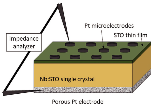
Figure 13. Sketch of a typical sample for electrochemical characterization with a (doped or nominally undoped) SrTiO 3 thin film on a Nb-doped SrTiO 3 substrate. For well-defined electrical contact, circular Pt microelectrodes (300 \mu\text{m} in diameter) are deposited on top of the SrTiO 3 thin film. A porous Pt layer acts as the counter electrode at the bottom of the Nb-doped SrTiO 3 single crystal.
