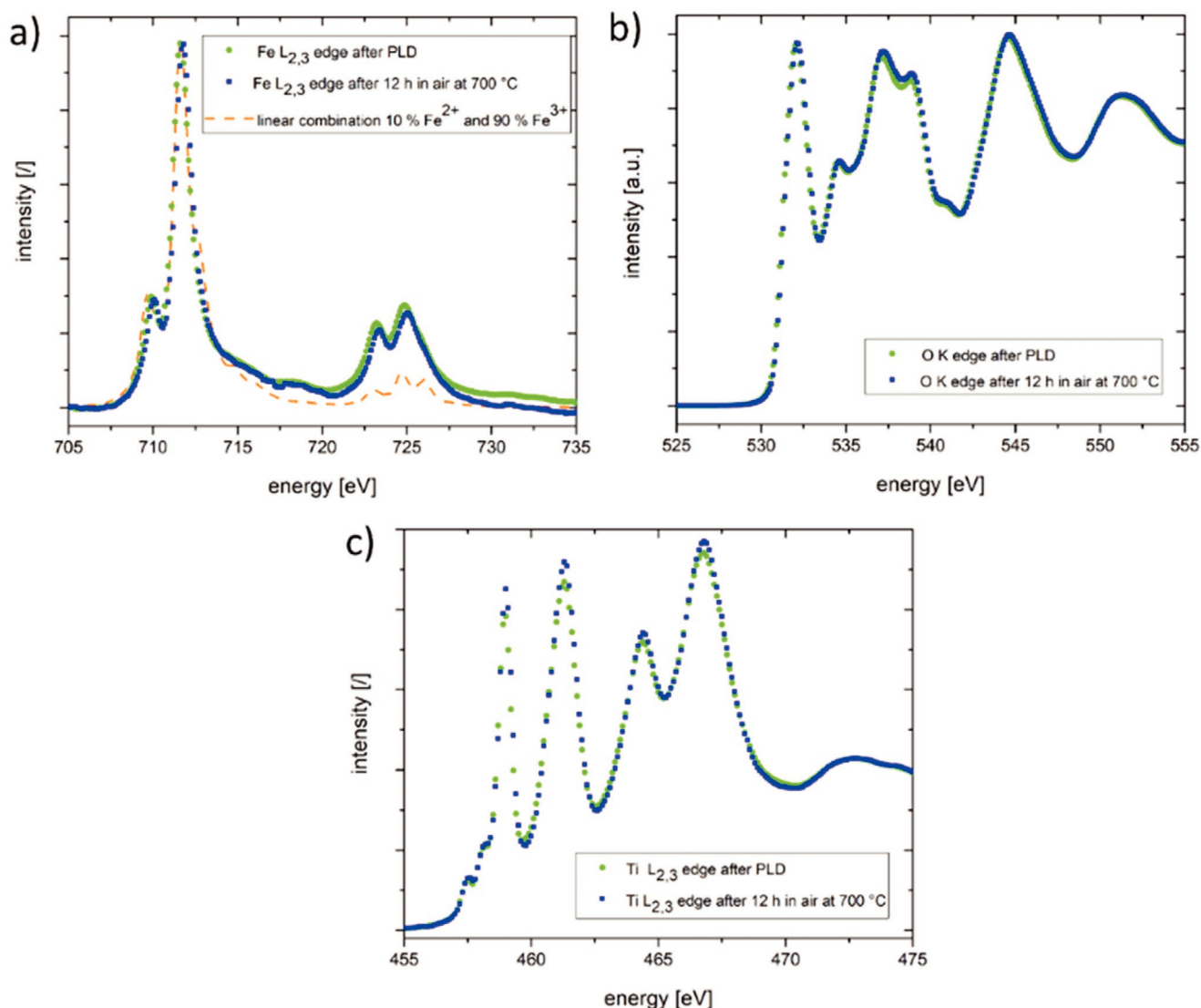
Figure 6. X-ray absorption measurements in fluorescence mode showing the a) Fe L 2,3 -edge, b) O K-edge, and c) Ti L 2,3 -edge of Fe-doped SrTiO 3 thin films deposited from a stoichiometric target with 2% Fe directly after the pulsed laser deposition (green dots) and after an additional annealing step at 700 °C in air for 12 h (blue squares). A linear combination of 10% Fe 2+ and 90% Fe 3+ (orange dashed line) matches the experimental data best.
