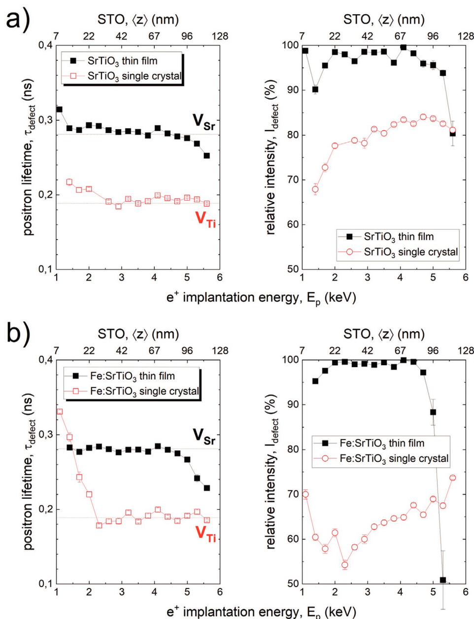
Figure 4. Positron lifetime annihilation spectroscopy (PALIS) measurements to reveal the types of point defects present in thin films and single crystals. a) The most dominant point defects found in a nominally undoped \text{SrTiO}_3 thin film are compared to those of a nominally undoped \text{SrTiO}_3 single crystal. b) Results for a thin film deposited from a 2% Fe-doped \text{SrTiO}_3 target are contrasted with the respective defects found in an Fe-doped single crystal with 0.15% Fe. A significant change in the defects found in thin films and single crystals can be observed for both cases. In thin films, Sr vacancies are the dominant point defect, whereas in single crystals titanium vacancies are identified.
