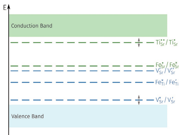
Figure 8. Suggested band structure of our pseudo-intrinsic Fe-doped SrTiO 3 thin films. Fe at the B-site (Fe Ti •• /Fe Ti •• ) works as an acceptor. We suggest V Sr •• /V Sr •• states in the middle of the band gap. Site changes caused by Sr vacancies lead to donor states. Most important is Ti on the A-site, Ti Sr •• /Ti Sr •• , corresponding to shallow donor states. The levels corresponding to Fe Sr defects are deep donors, slightly above mid-gap. Sr vacancies also act as acceptor states close to the conduction band (V Sr •• /V Sr •• ). Arrows indicate that the position of several states in the band-gap is a first estimate; our model does not depend on their exact position (within a certain range).
