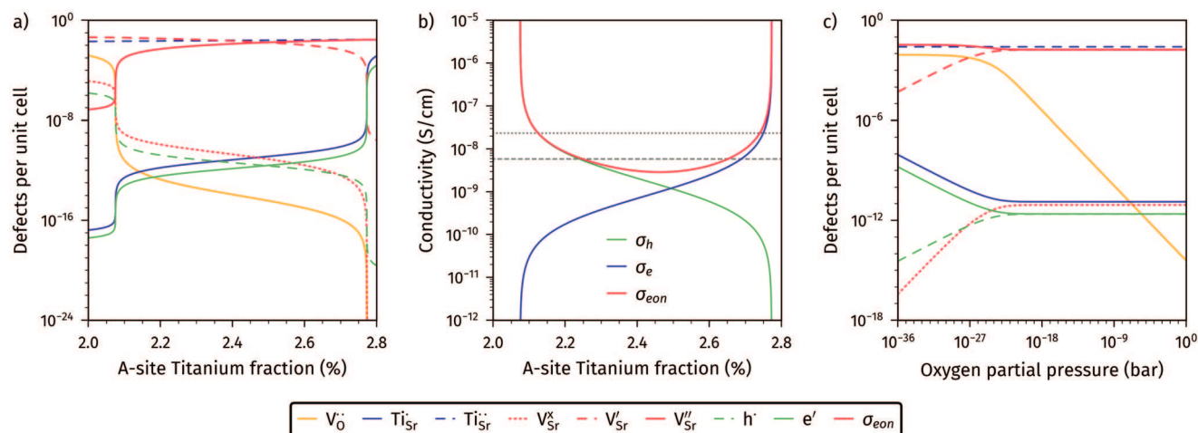
Figure 9. Defect chemical calculations at 400 °C for the defect chemical parameters in Table 2 and Ref. [1]. (a) Defect concentration against A-site Ti fraction, constrained to the elemental composition determined by ICP-OES, i.e. Sr/Ti = 0.918 and p_{\text{O}_2} of 1 bar. (b) Corresponding electron, hole and sum conductivities. (c) A Brouwer diagram for Sr deficient undoped \text{SrTiO}_3 with Ti partly on the A site ( \text{Sr}_{0.941}\text{Ti}_{1.025}\text{TiO}_{3-\delta} ).
