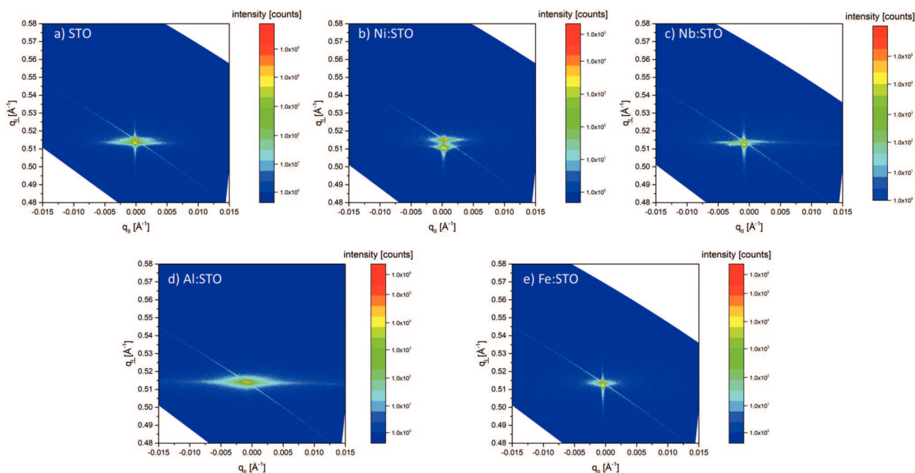
Figure 3. Structural characterization of different SrTiO 3 thin films on top of nominally undoped (001) oriented SrTiO 3 single crystals. a) Thin films were deposited from nominally undoped, b) 0.4% Ni-doped, c) 2% Nb-doped, d) 0.3% Al-doped, and e) 1% Fe-doped SrTiO 3 targets. Here, reciprocal space maps (RSM) for the (002) reflections are shown, revealing a severe deviation in the lattice parameter for the thin films compared to the underlying SrTiO 3 substrates. Except for the Al-doped thin film (d) the out of plane cell parameter c from each of the prepared thin films is elongated compared to the substrate. As a consequence, in the RSMs two separated reflexes can be found. The deviation between the thin film and the substrate can be attributed to cation vacancies. Taking the Sr deficiency found by elemental analysis into account, the cation vacancies are identified as Sr vacancies.
