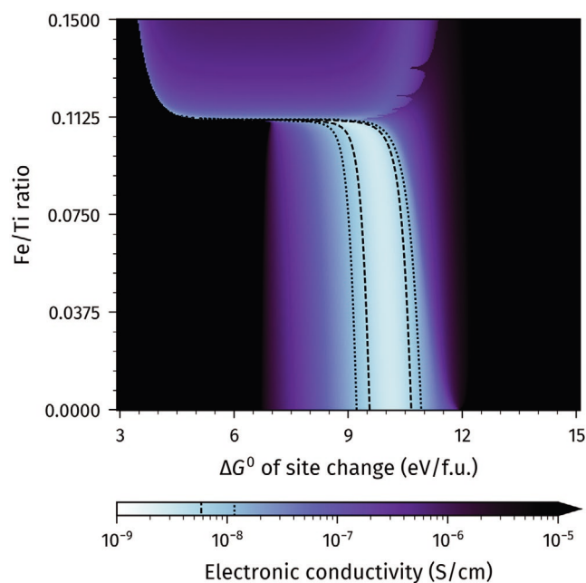
Figure 12. Electronic conductivities at 400 °C, p_{O_2} = 1 bar, compared to the intrinsic conductivity for different \Delta G^0 values, Sr vacancies being exactly mid-gap and the Fe doping level varying while Sr/(Fe+Ti) is fixed at 0.90 and Fe_{Sr} is neglected here. In a broad range of Fe doping levels the pseudo-intrinsic situation again results as long as \Delta G^0 is between 9.5 and 10.5 eV.
