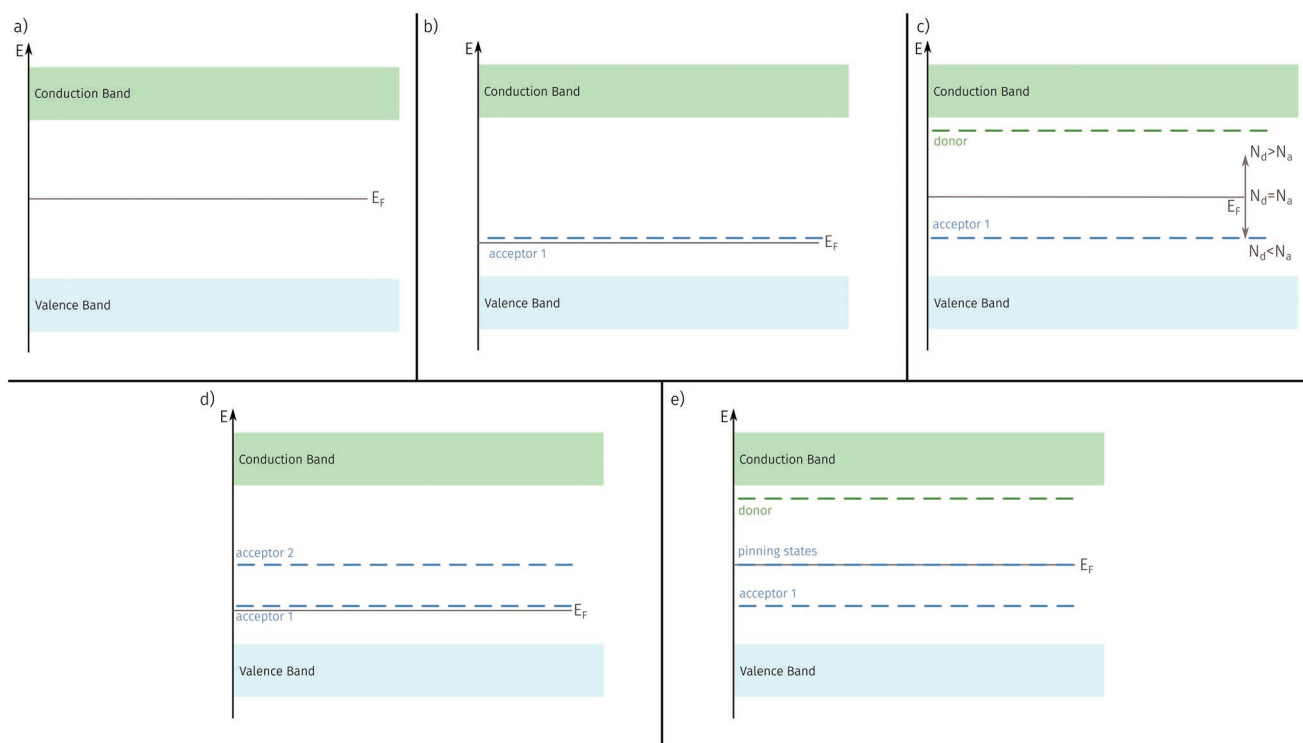
Figure 7. Band structure of SrTiO 3 for different doping cases. a) Fermi level is mid-gap, corresponding to intrinsic concentrations in a semiconductor. This is the hypothetical case of ultra pure, defect-free, stoichiometric SrTiO 3 . b) With the introduction of acceptor states (acceptor 1), the Fermi energy is adjusted accordingly. Here a deep acceptor is shown, with both acceptor and donor dopants present. c) For exactly equal amounts of acceptor and donor states, the Fermi level is mid-gap. When the acceptor/donor ratio differs from unity, the Fermi level moves to the more dominant state. Hence, the Fermi level is not pinned at mid-gap in a robust manner. d) If instead of the donor in (c) a mid-gap acceptor (acceptor 2) is added, the Fermi level is mostly dominated by the acceptor 1 states. e) Both acceptor (acceptor 1), donor, and mid-gap states (acceptor 2) are present, allowing robust mid-gap Fermi level pinning.
