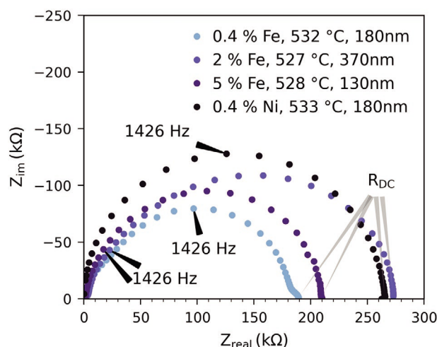
Figure 1. Electrochemical characterization of different SrTiO 3 thin films deposited from targets with 0.4%, 2%, and 5% Fe as well as 0.4% Ni doping. The measurement temperatures deviate slightly for the individual samples, but are all in the range of 527–533 °C. Film thicknesses are in the range of 130–370 nm. The DC resistances of the main arcs ( R_{DC} ) and the 1426 Hz data points are indicated for the different impedance spectra. The DC resistances are in the range of 180–280 kΩ. Different degrees of distortion can be identified, for example, nearly undistorted for 0.4% Ni to heavily distorted for 2% Fe doping.
