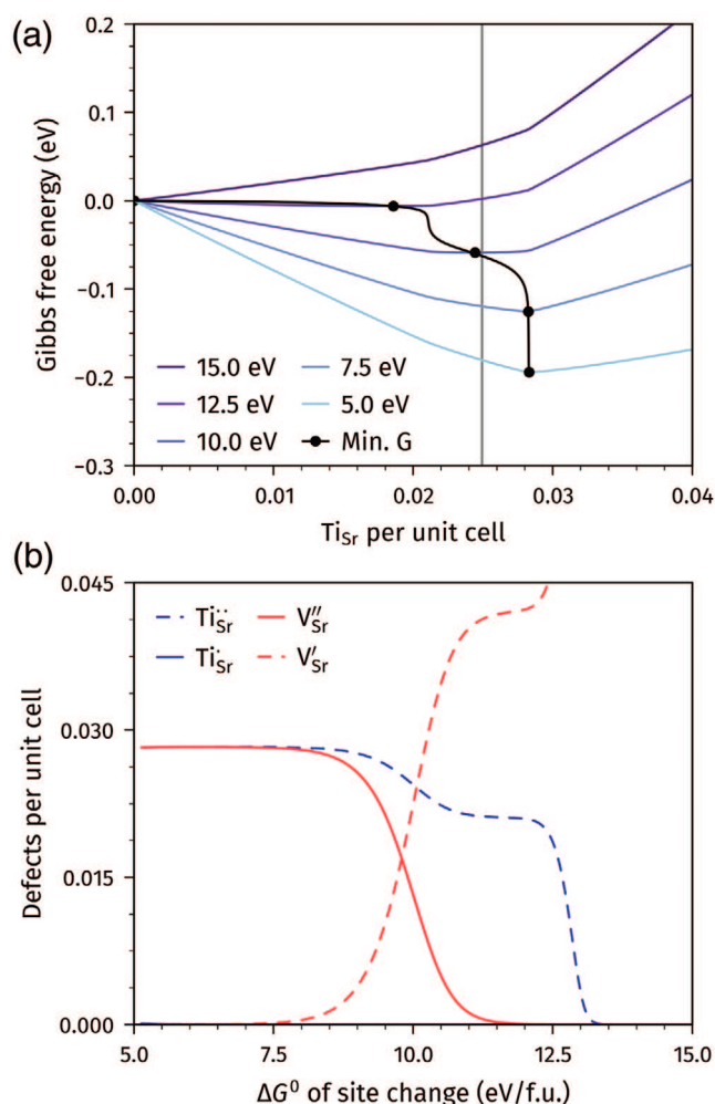
Figure 10. (a) Gibbs free energy G of an undoped \text{SrTiO}_3 film with \text{Sr}/\text{Ti} = 0.918 calculated for a progressing site change reaction, Equation 8, at 650^\circ\text{C} and 0.15\text{mbar} oxygen partial pressure and different standard Gibbs energies of the reaction \Delta G^0 . In a certain range, the minima of G correspond to \text{Ti}_{\text{Sr}} values with pseudo-intrinsic conductivities. (b) Dependence of several equilibrium donor and acceptor defect concentrations on the standard Gibbs free energy of the site change reaction.
